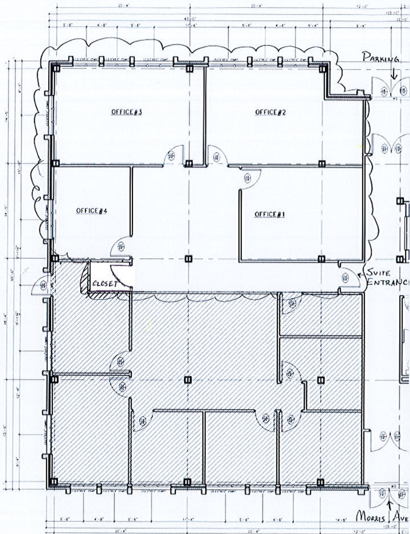
1 FIRST FLOOR PLAN A-1 EXISTING SCALE 1/4"=1'-0"
