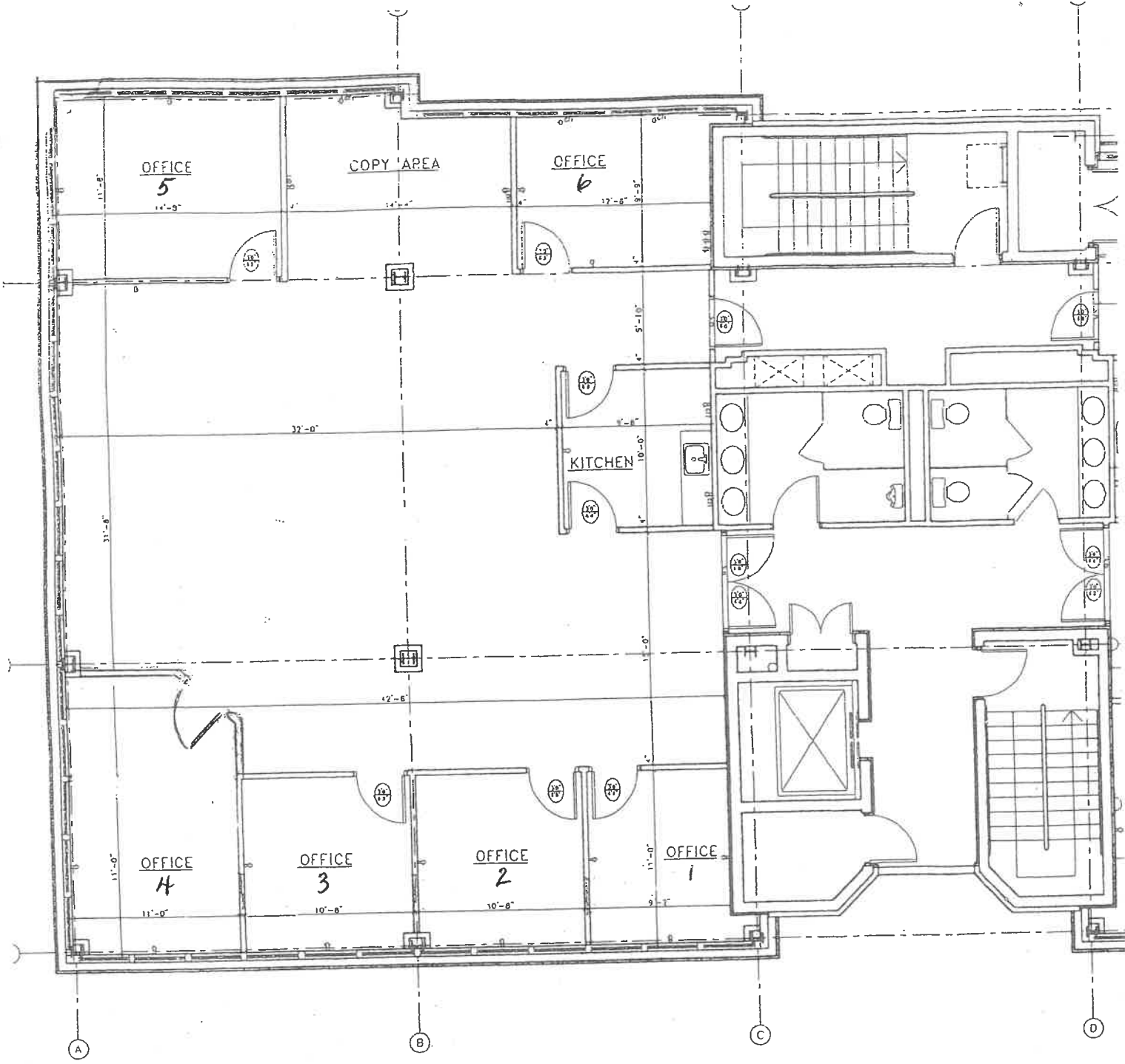
1 FLOOR PLAN A-1 SCALE 1/8" = 1'-0"
